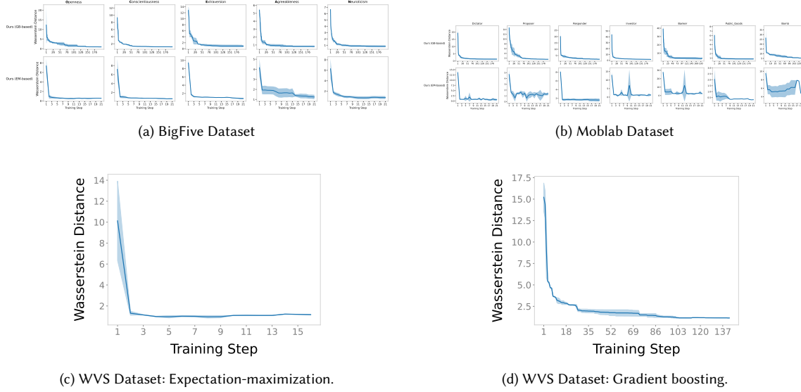
Fig. D.1. Algorithm convergences on the Big Five and MobLab datasets.
